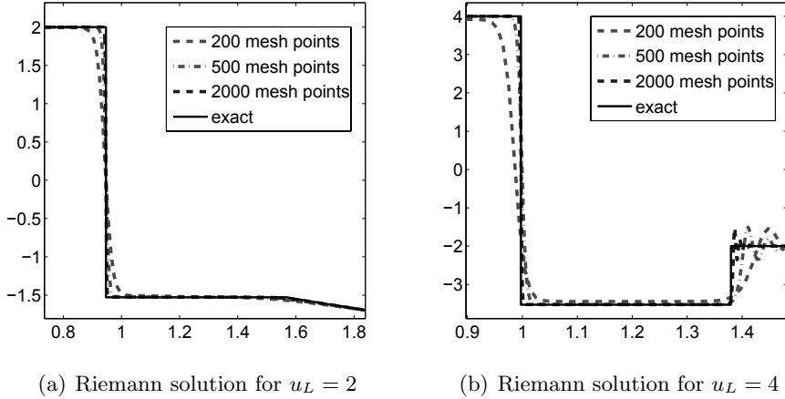
Figure 3.4. Convergence (mesh refinement) for the WCD schemes and small shocks. All approximations are based on an eighth-order scheme and \tau = 0.01 .
